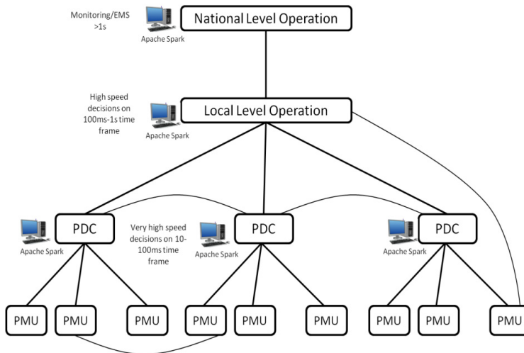
Fig. 4. PDUs embedded with Apache Spark at different levels
